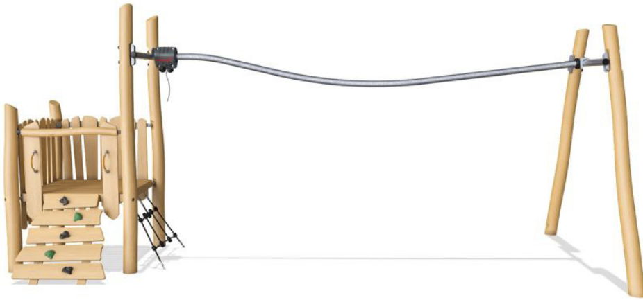
Track Ride Tower NR01027 www.kompan.com main materials: FSC certified hardwood and galvanised steel Age Range 6-12 years BS EN 1176
